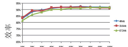
DDR-120C-48
