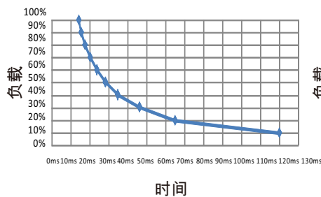
DDR-120D-24
