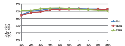
DDR-120B-48
